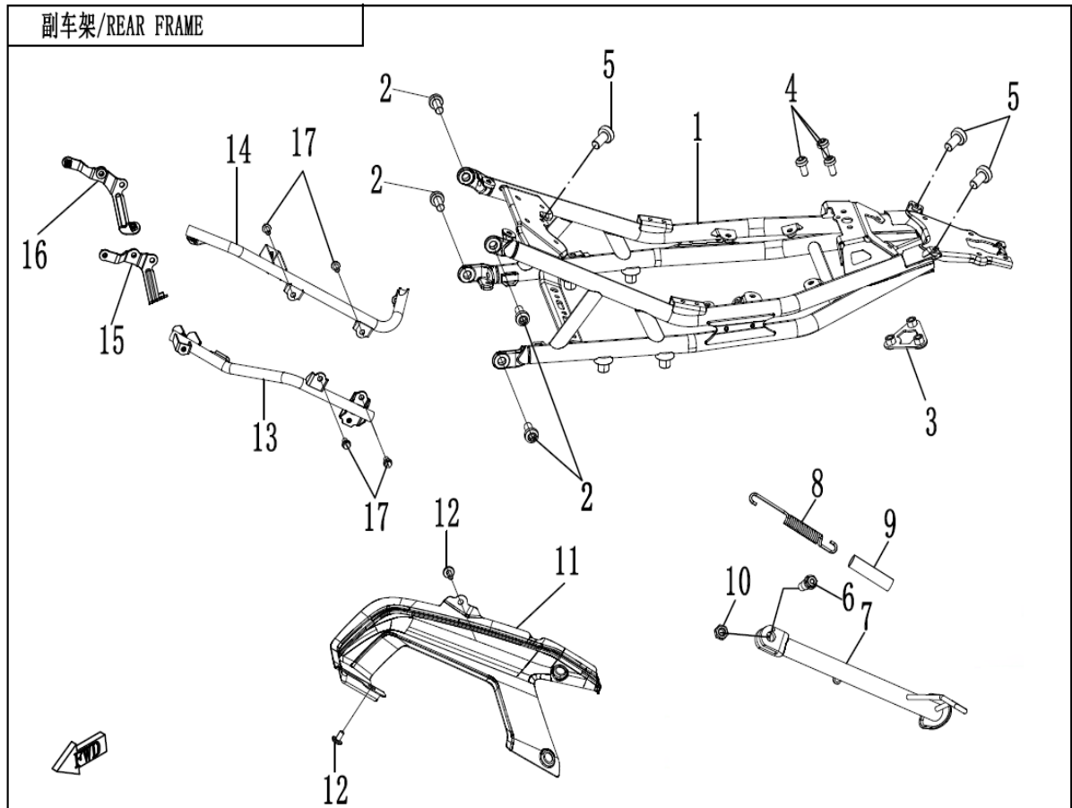
F03-2 REAR FRAME
