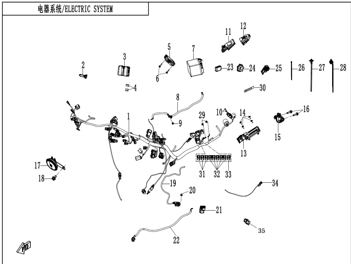
F15 ELECTRIC SYSTEM
