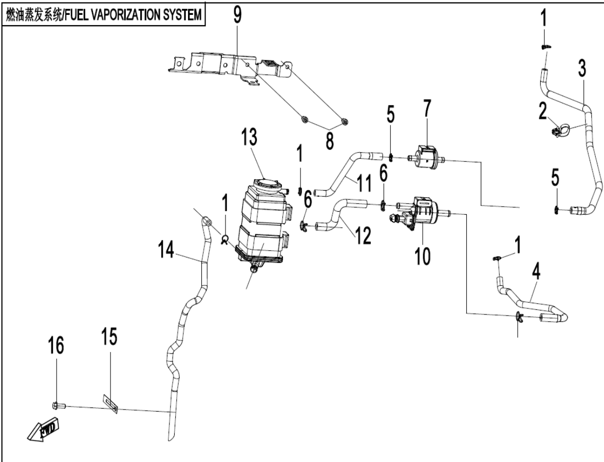
F36 FUEL VAPORIN SYSTEM
