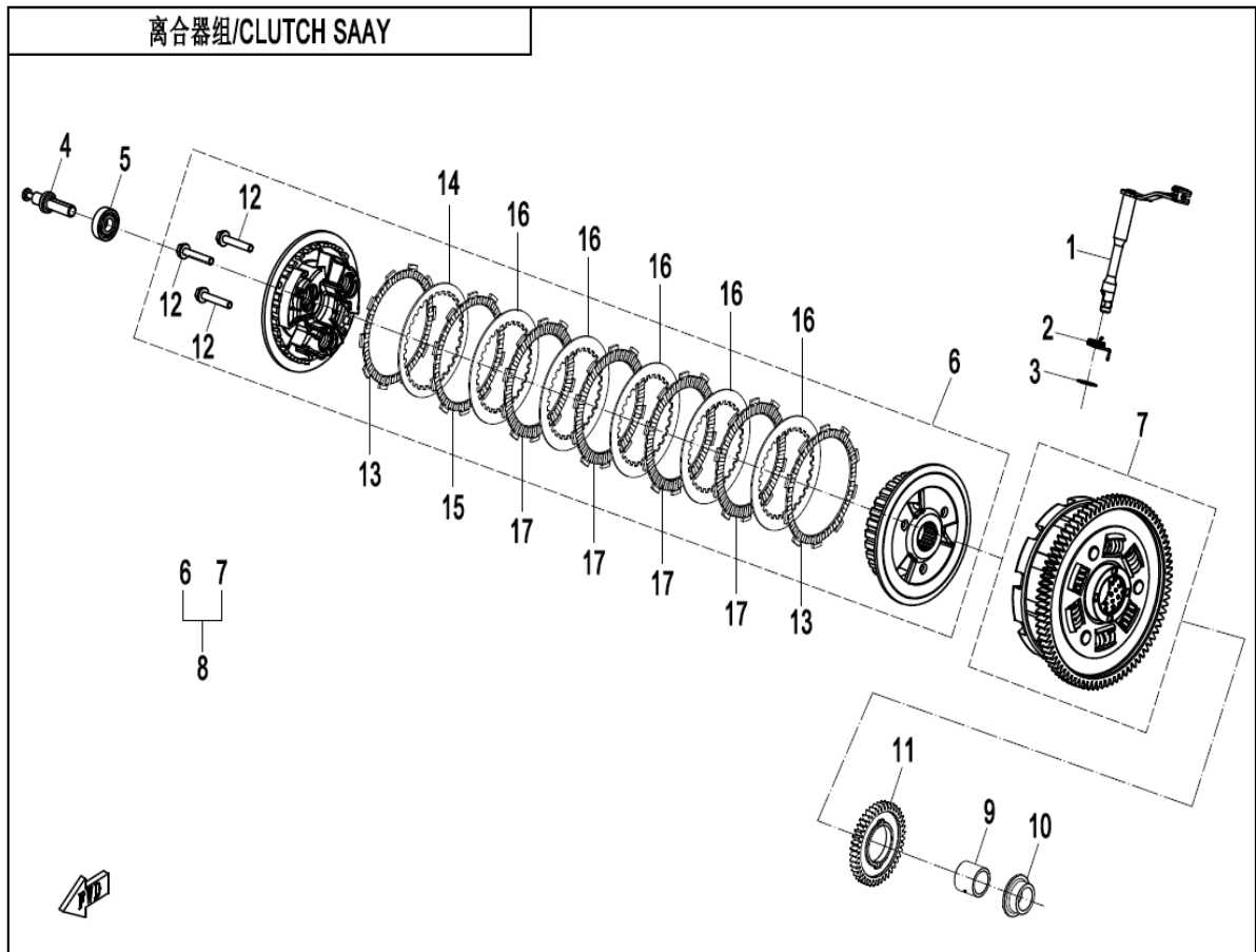
E05 CLUTCH ASSY
