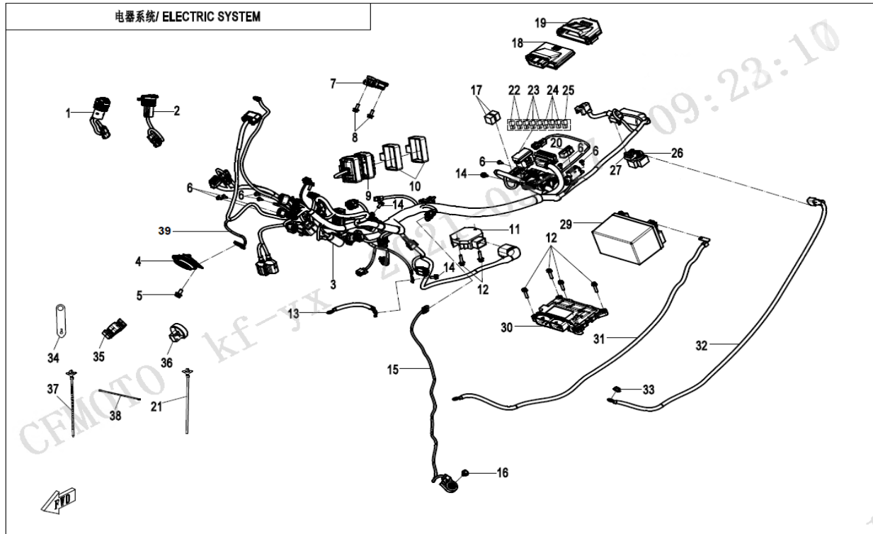
F15-1-B ELECTRIC SYSTEM(TOURING)
