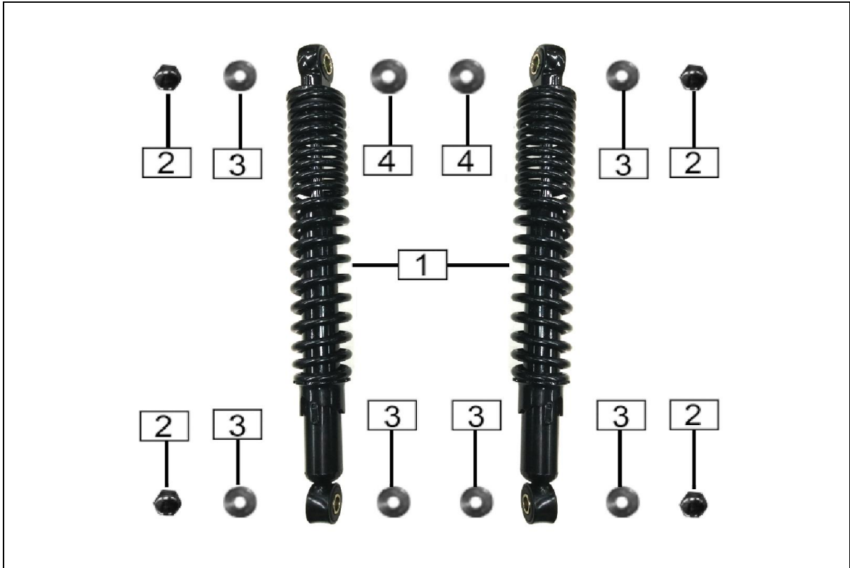
F27 REAR SHOCK ABSORBER
