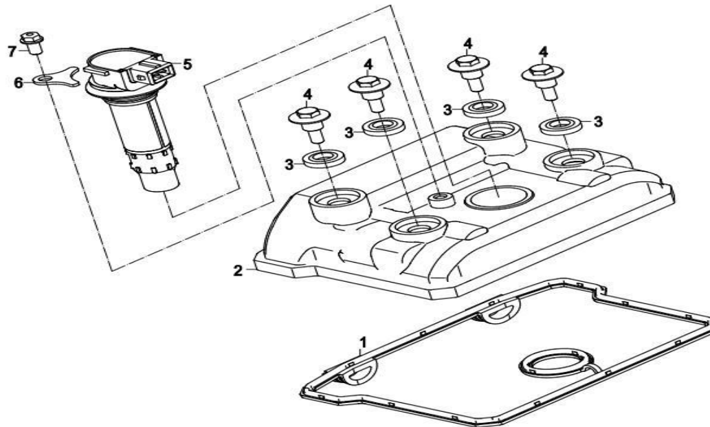
CYLINDER HEAD COVER
