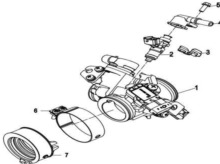
THROTTLE & INJECTOR
