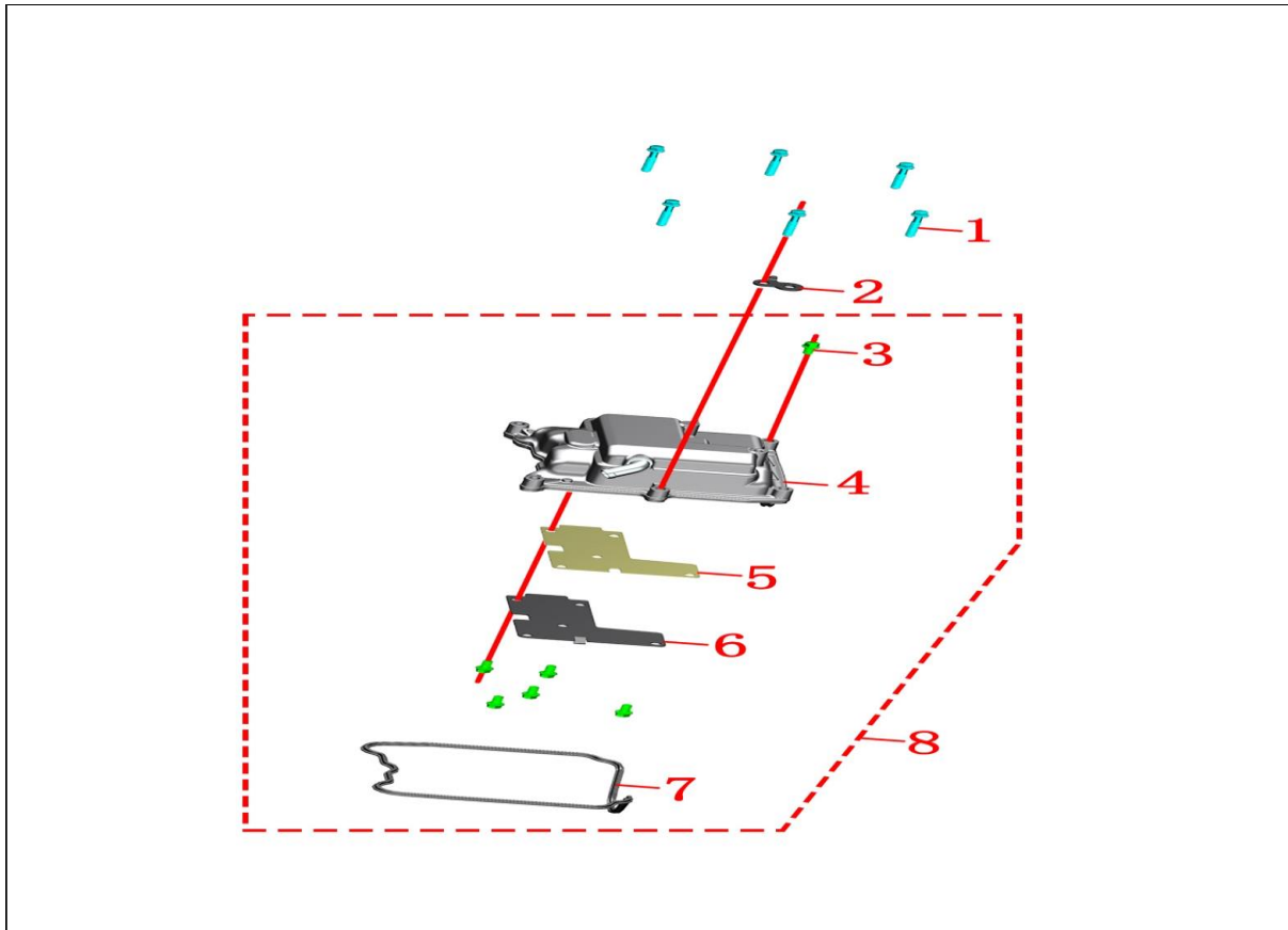
E-01 CYLINDER HEAD COVER SUB-COMPONENTS (LONG WHEELBASE VERSION)
