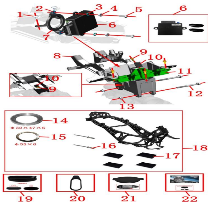
F-17 HEAD BRACKET ASSEMBLY
