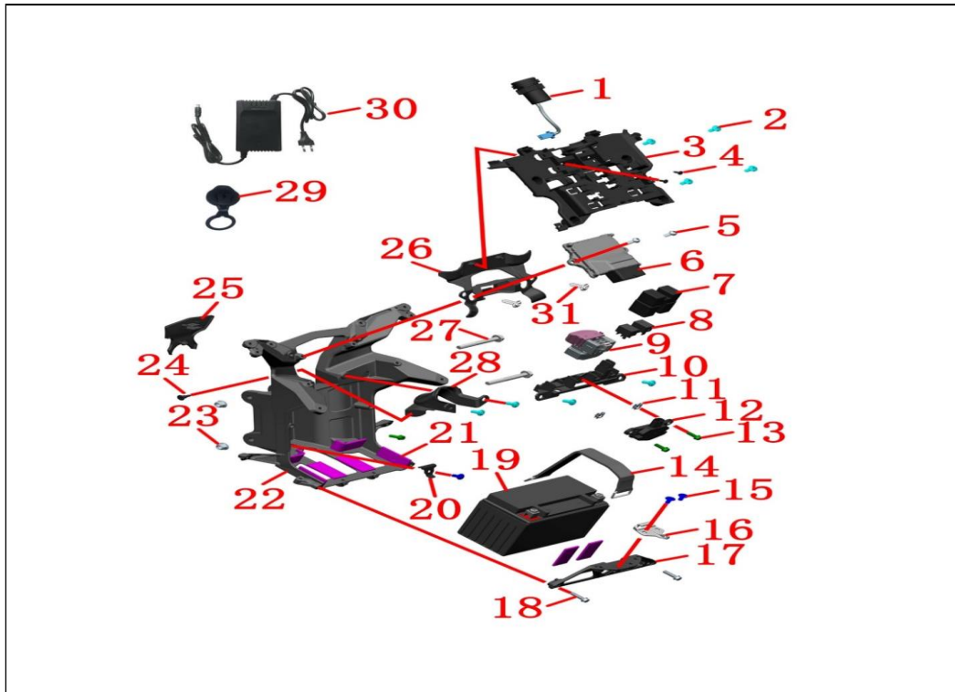
F-35 HEADREST/BATTERY/ECU ASSEMBLY (1/2)
