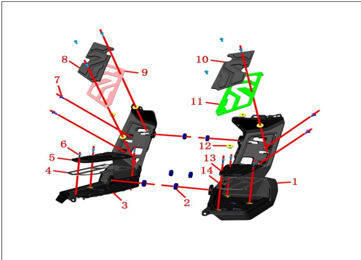
F-13 PEDAL ASSEMBLY
