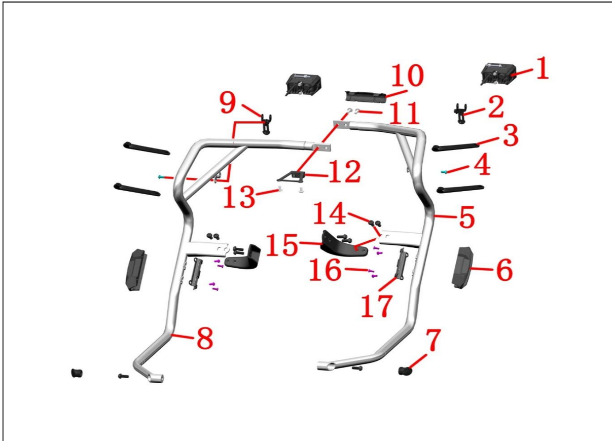
F-24 BUMPER GUARD - FOG LIGHT ASSEMBLY (LOW FOOT PEDAL) I
