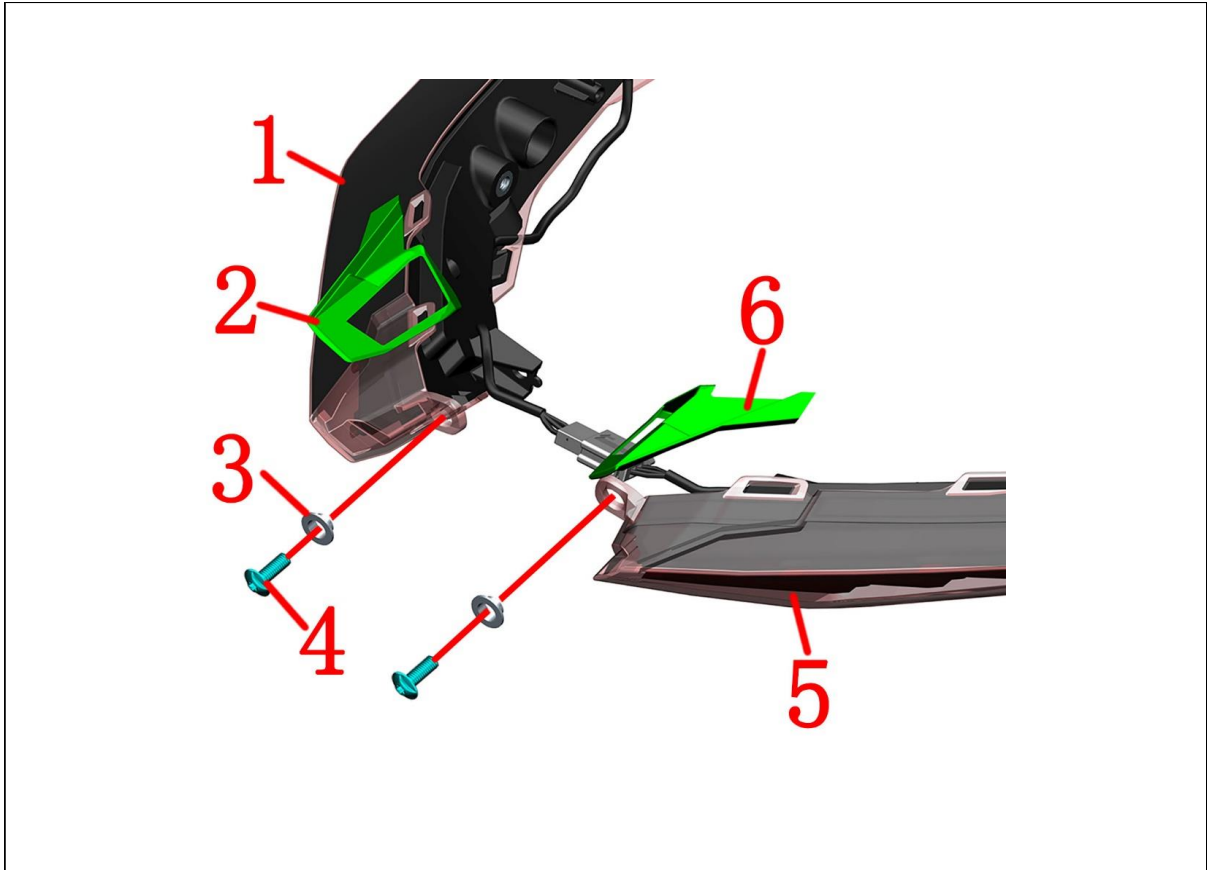
F-22 TAILLIGHT ASSEMBLY
