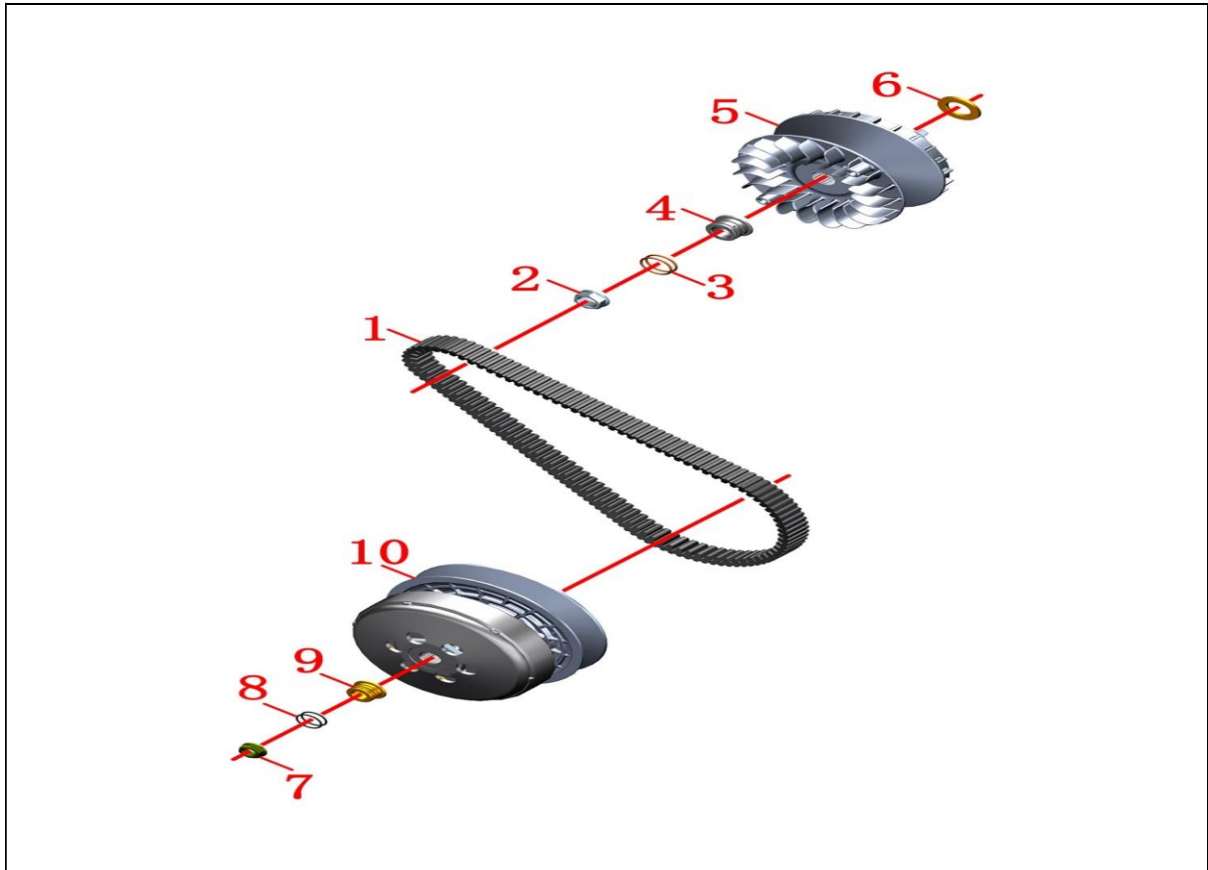
E-06 CONTINUOUSLY VARIABLE TRANSMISSION (CVT) SUB-ASSEMBLY
