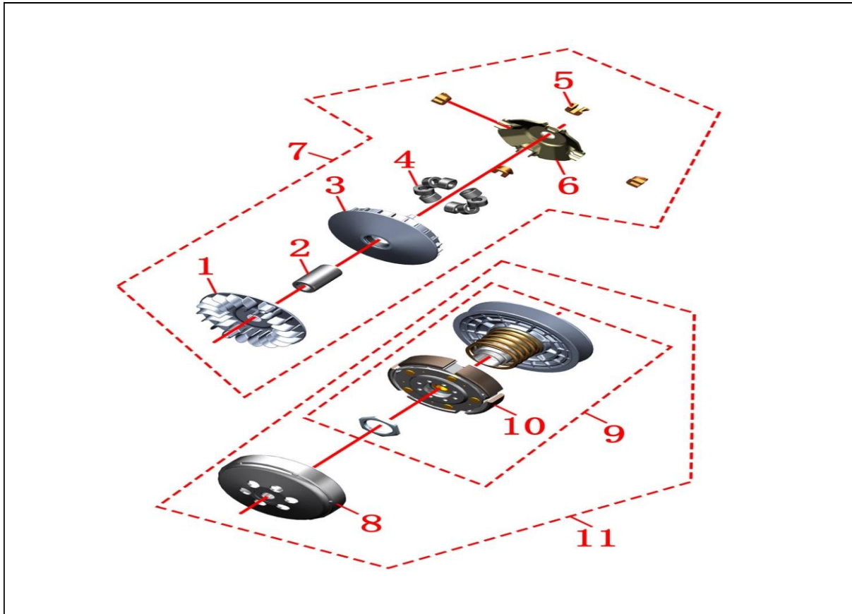
E-07 CONTINUOUSLY VARIABLE TRANSMISSION (CVT) CLUTCH SUB-ASSEMBLY
