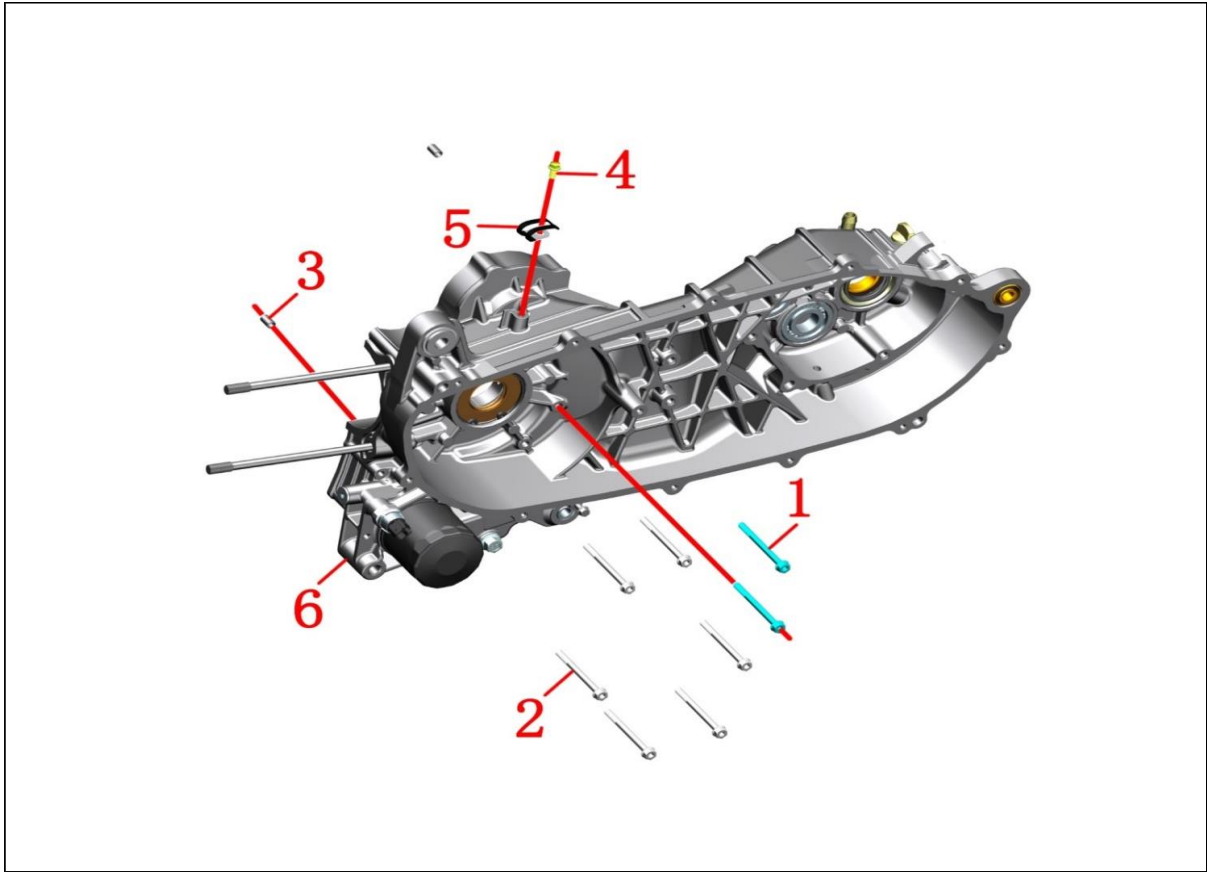
E-09-01 LEFT CRANKCASE SUB-ASSEMBLY (LONG WHEELBASE)
