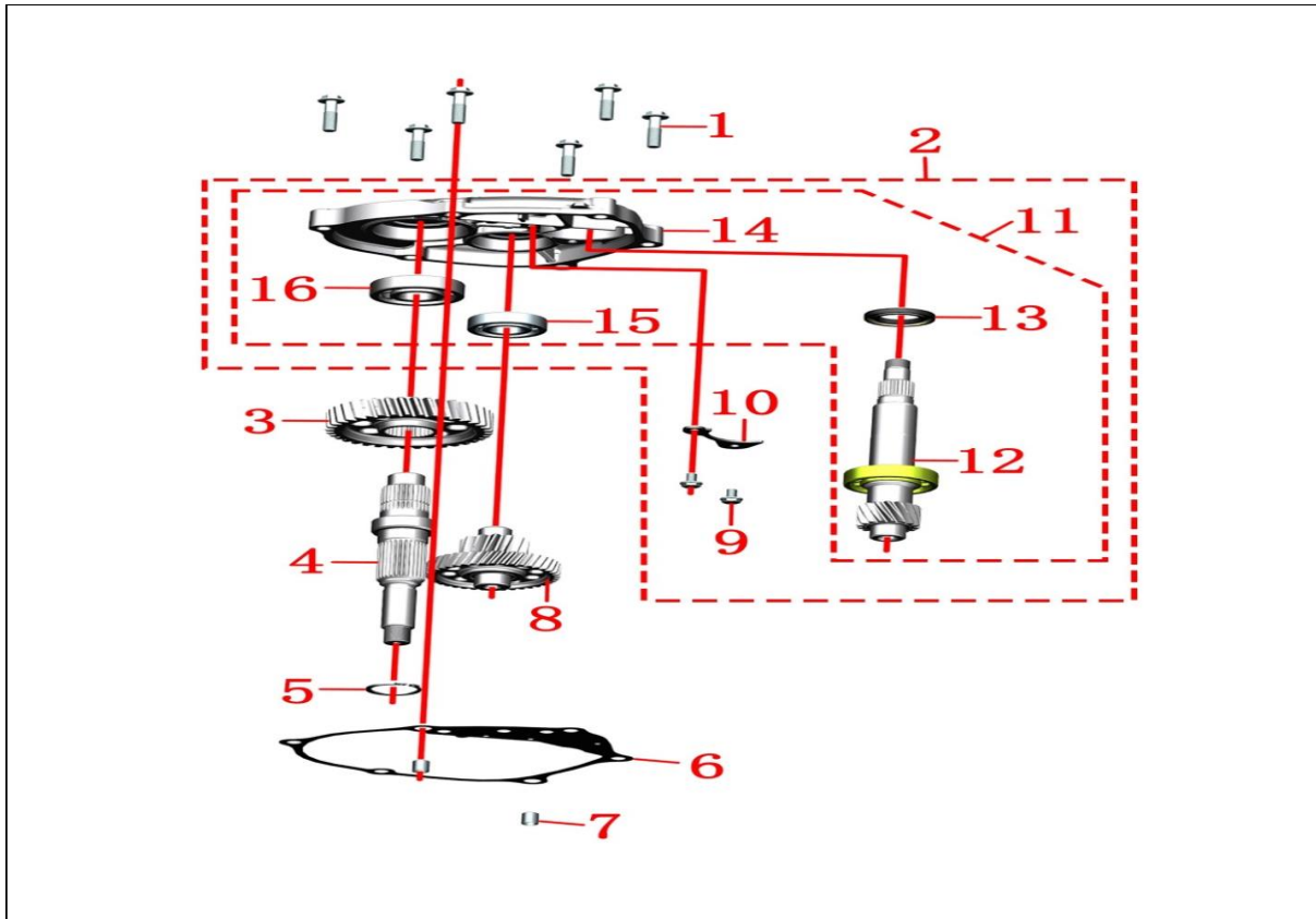
E-11 GEARBOX COVER SUB-ASSEMBLY
