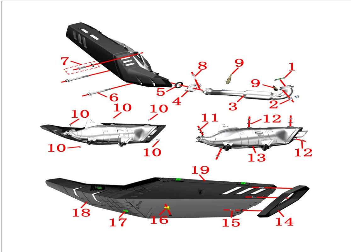
F-44 MUFFLER ASSEMBLY
