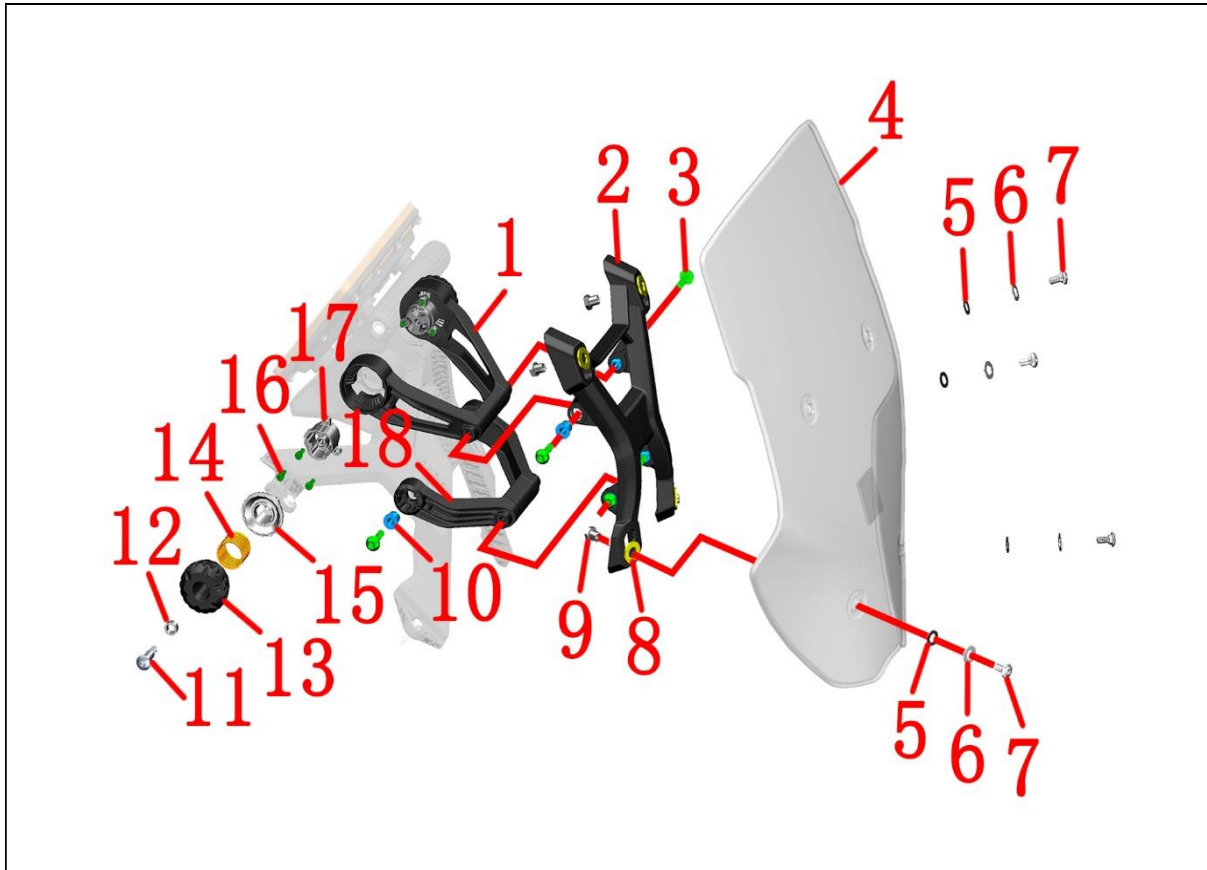
F-01 INSTRUMENT PANEL WINDSHIELD ASSEMBLY 1
