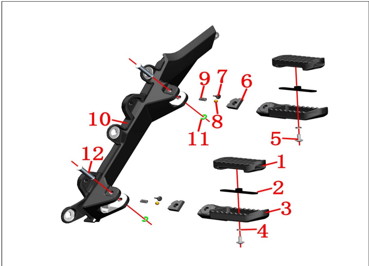
F-46 LEFT PEDAL ASSEMBLY
