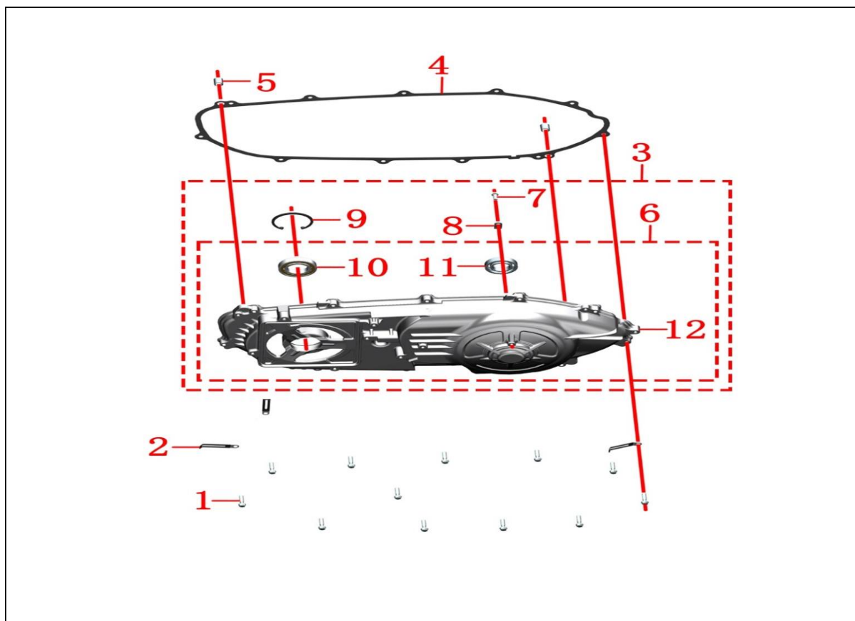
E-12 LEFT CRANKCASE COVER A SUB-ASSEMBLY
