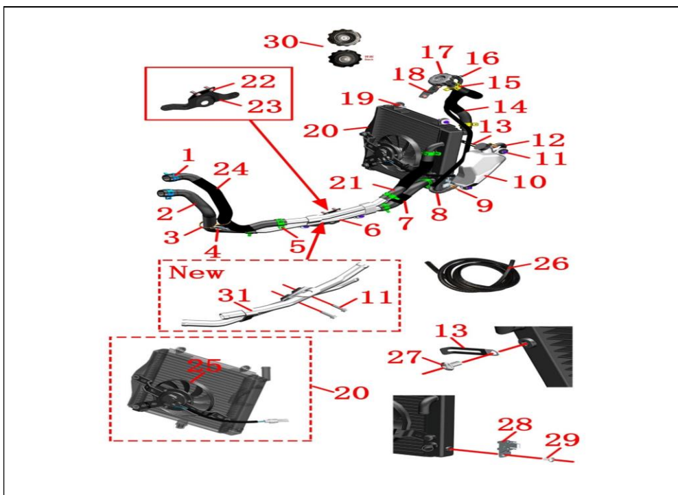
F-48 COOL SYSTEM ASSEMBLY
