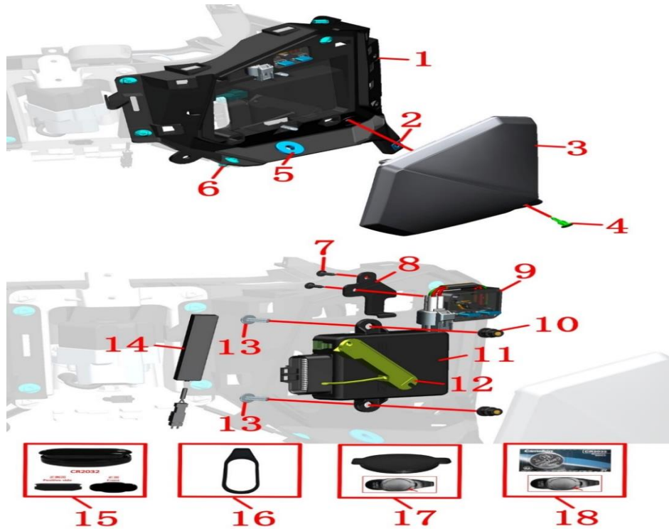
F-09 FRONT STORAGE BOX COVER ASSEMBLY 4
