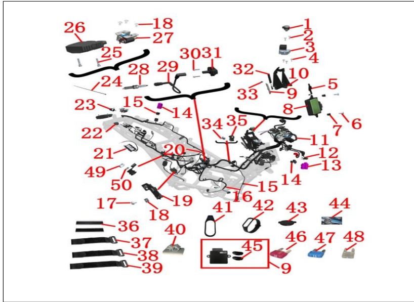
F-36 ELECTRIC PARTS ASSEMBLY
