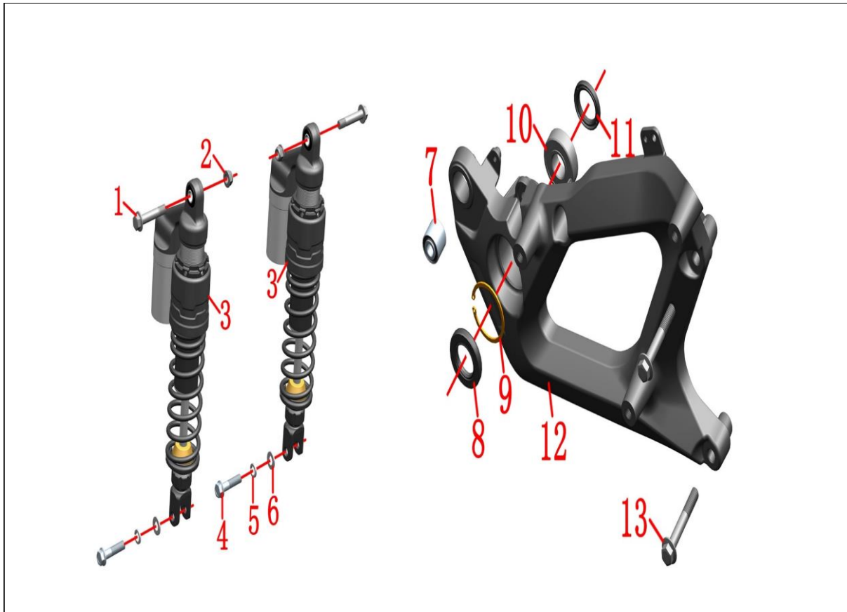
F-32 REAR SHOCK ABSORBER ASSEMBLT (HIGH SEAT)
