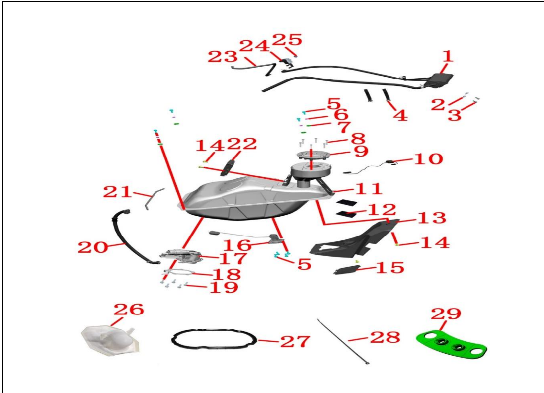
F-37 FUEL TANK ASSEMBLY (FROSTED SILVER FUEL TANK LOCK)
