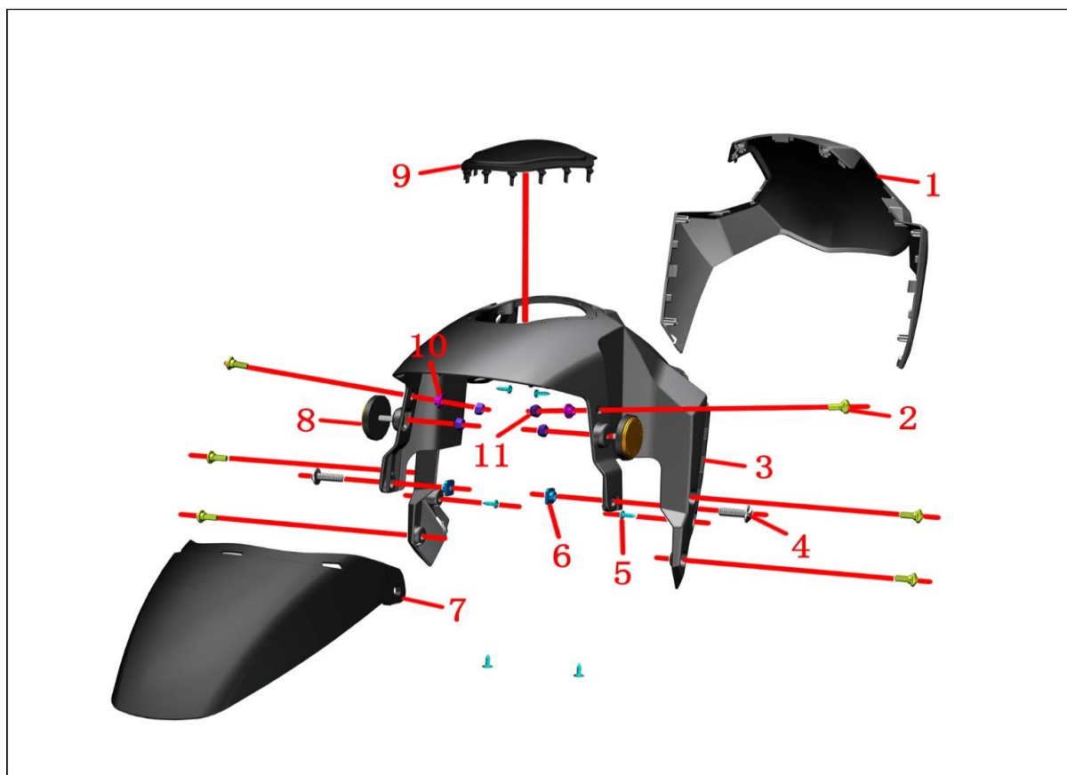
F-25 FRONT FENDER ASSEMBLY
